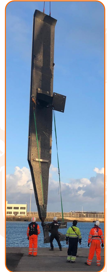
Harbor fender installation
