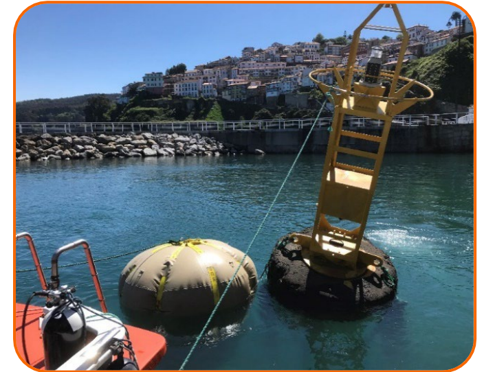
Buoy towing and anchoring
