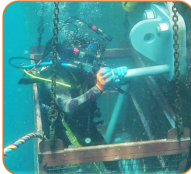
Installation of harbor fenders
